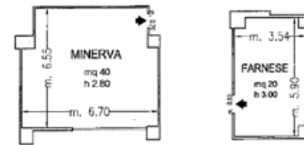
Piano Terra / Ground Floor
